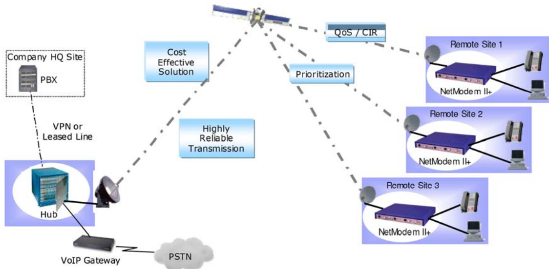
Figure 1: iDirect VoIP Solution
